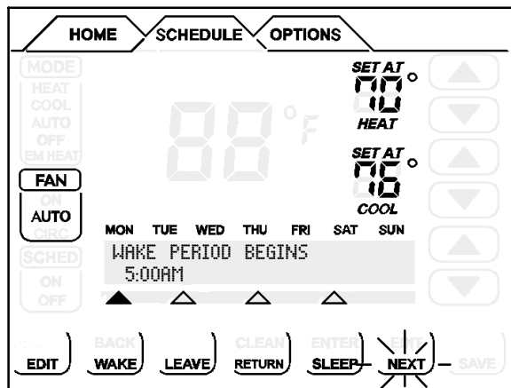
Figure 4. Schedule Screen
